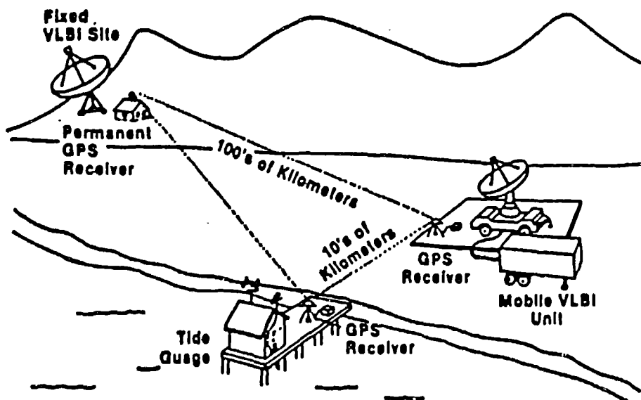
Fig. 12 Proposed link of tide gauges and geodetic controls
