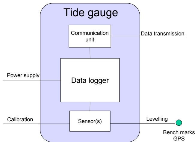
Figure 15. Tide gauge.
