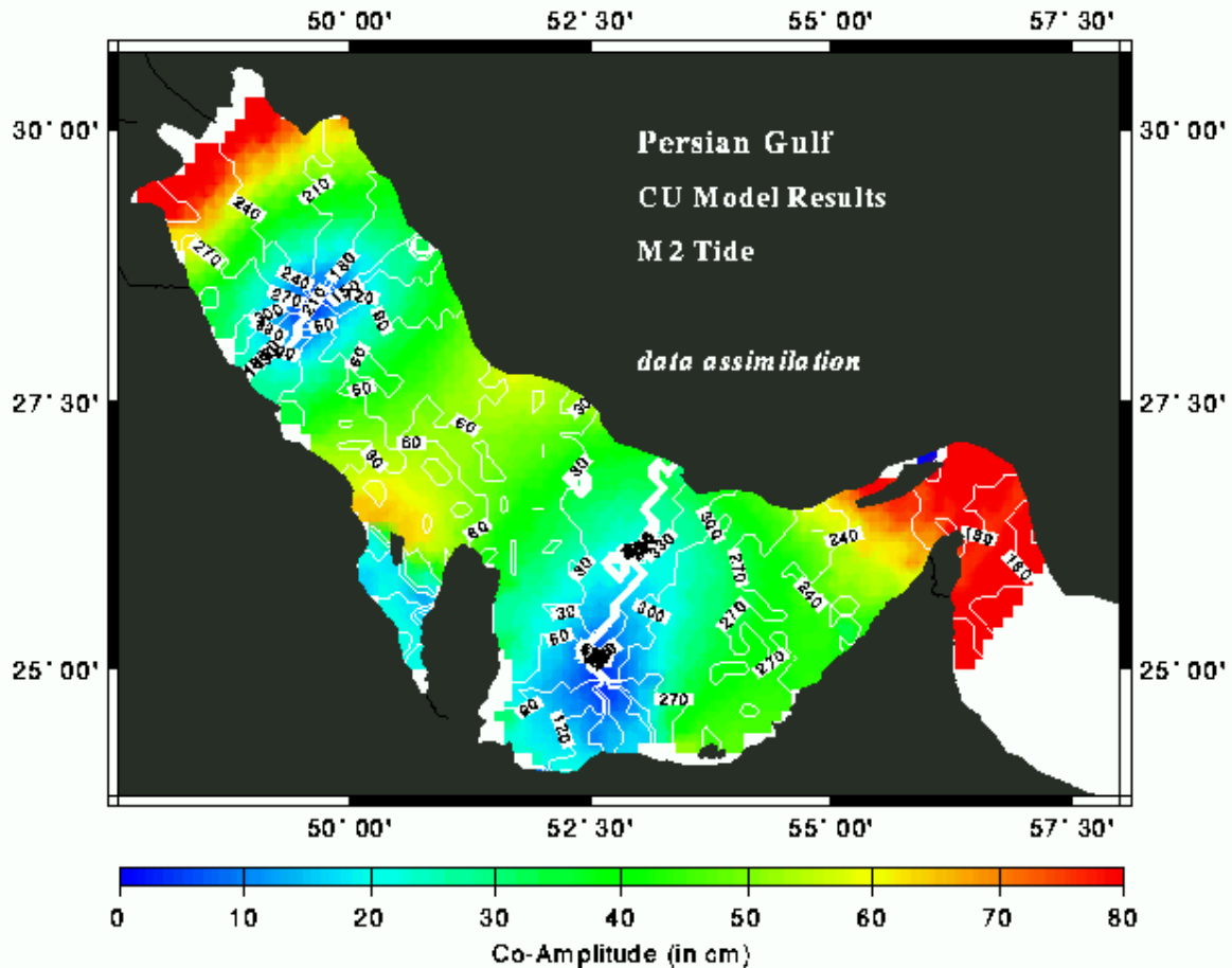
Figure 2. The Persian Gulf M2 tide derived from the CU/NAVOCEAN model using data assimilation of tide gauges. 18 km resolution on an inclined grid. Source: Naval Oceanographic Office.
