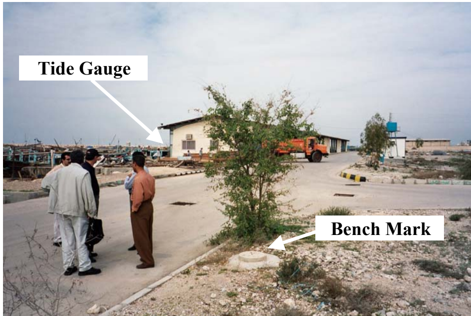
Figure 5. Location of Tide Gauge and Bench Mark at Nakhl-e Taghi. The bench marks are located near the tide gauge and are tied into the Iranian levelling network.
