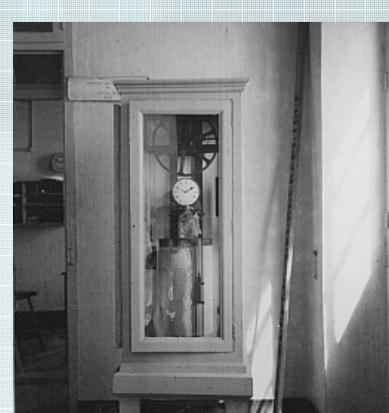
Figure 3. View of the recording drum and clock of the mechanical floating tide gauge at Dakar (SHOM, 1959).
