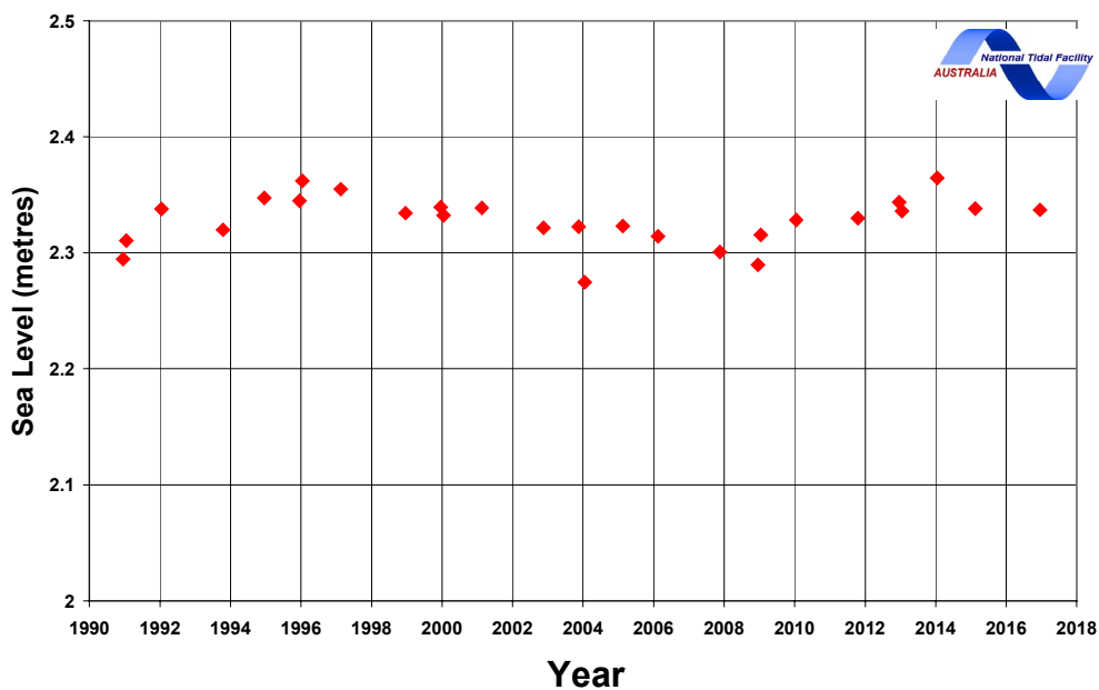
Predicted highest tide each year for Lautoka
